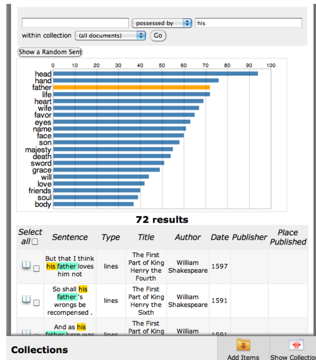
Figure 4: Grammatical search results for possessed-by his , filtered on the word father . Individual search results, corresponding to matching sentences, are highlighted to show the words in the relationship
